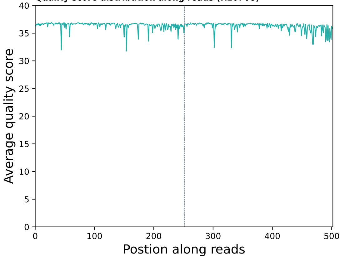
Quality score distribution along reads (R10708)
